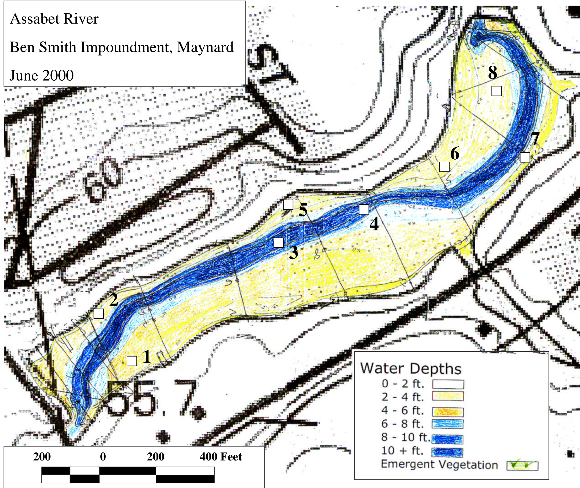
Figure 6-13 Sediment Nutrient Flux Survey Sampling Locations with Bathymetry of Ben Smith Impoundment, Maynard (RM 9.0)
